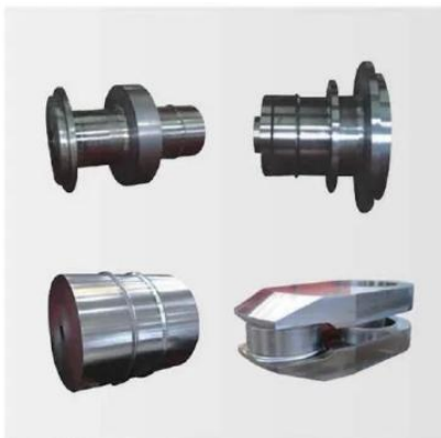
船用低速柴油机曲轴零件锻件 Forgings for crankshaft components of low-speed marine diesel engines
